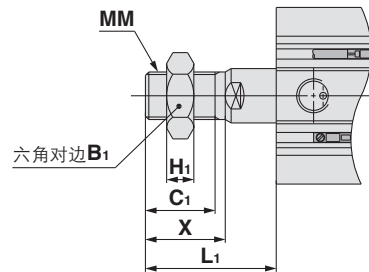
杆端外螺纹
