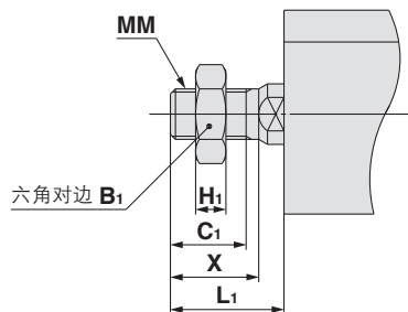
杆端外螺纹
