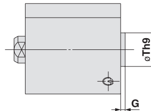
杆端外螺纹
