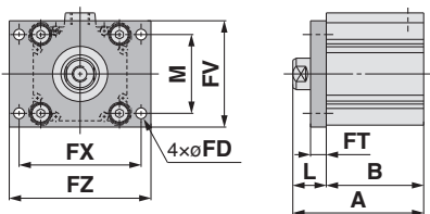
杆端外螺纹
